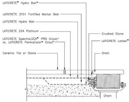
Detail 1 ES-WP301
