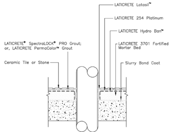
Detail 6 ES-WP300
