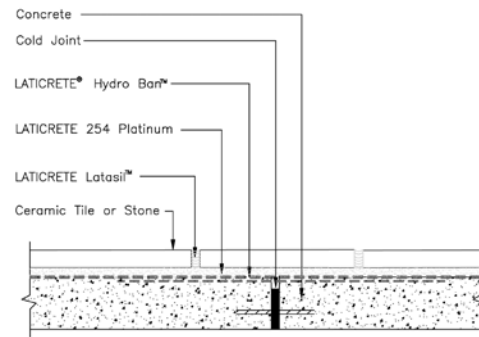
Detail 4 ES-EJ14
